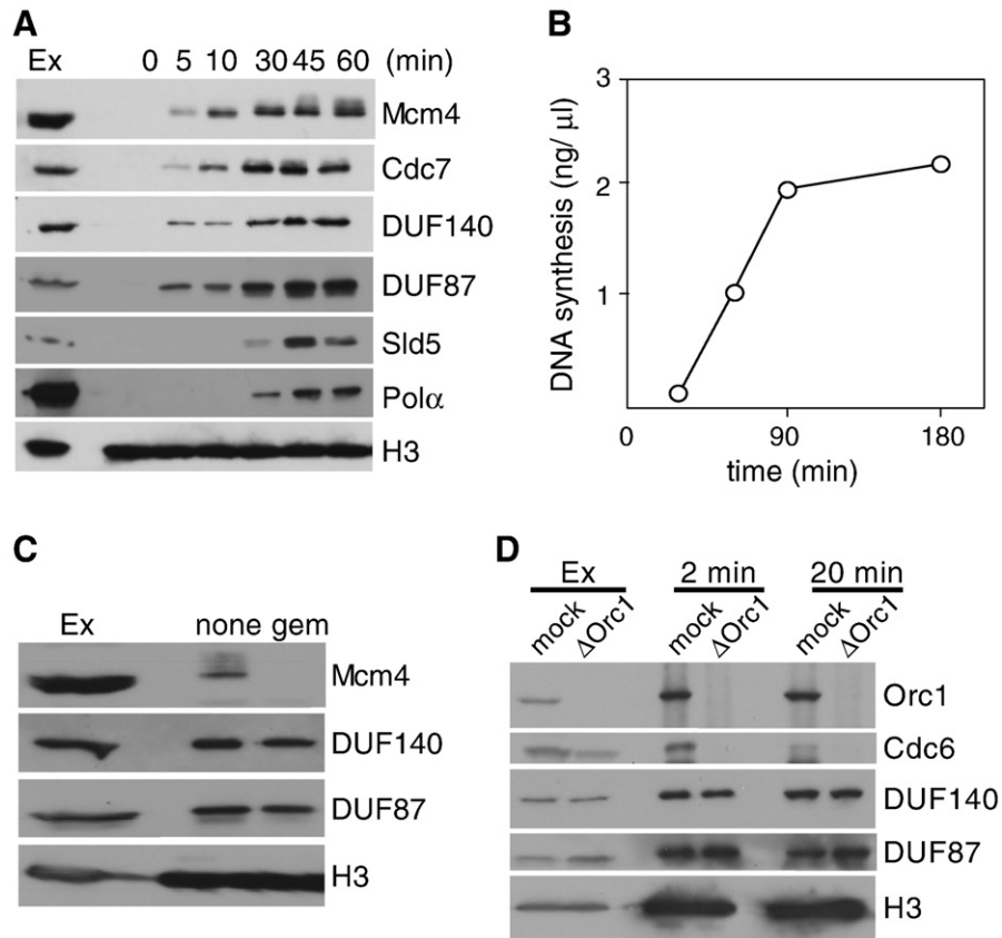
Fig. 1. FACT rapidly binds chromatin independently of origin licensing. (A) Sperm nuclei (7.5 ng DNA/μl) were incubated in extracts and isolated at indicated time points for immunoblotting. Egg extracts (Ex; 2 μl) were also applied. (B) Synthesized DNA at indicated time points was measured after incubation of sperm nuclei (3 ng DNA/μl) with Xenopus egg extracts. (C) Chromatin was isolated after incubation of sperm nuclei (7.5 ng DNA/μl) with extracts in the presence (gem) or absence (none) of geminin (100 nM). Isolated chromatin was subjected to immunoblotting. Egg extracts (Ex; 2 μl) were also applied. (D) Sperm nuclei (6 ng DNA/μl) were incubated for 2 or 20 min in mock-treated (mock) or Orc1-depleted ( \Delta Orc1) extracts. Isolated chromatin was subjected to immunoblotting. Mock-treated (mock) and Orc1-depleted ( \Delta Orc1) extracts (Ex; 2 μl) were also applied.
